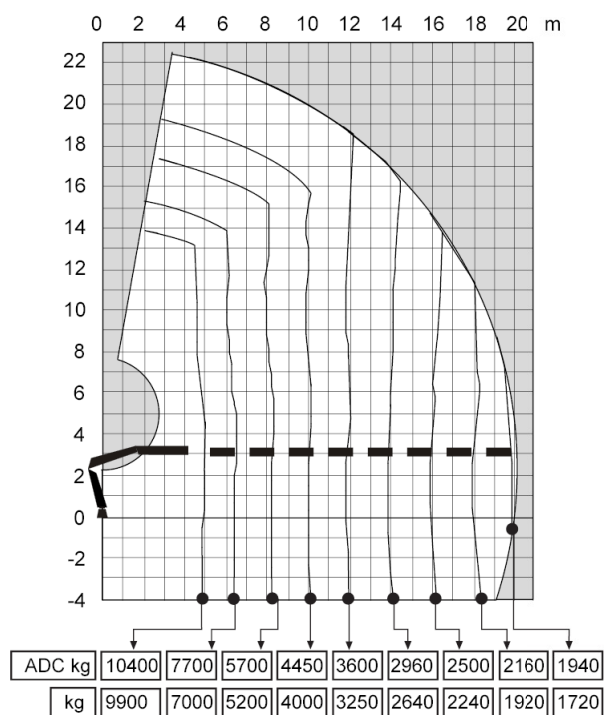
Load diagram
